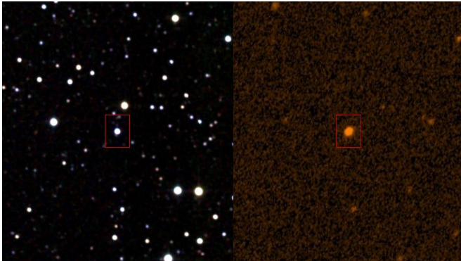
Star KIC 8462852 in infrared (2MASS survey) and ultraviolet (GALEX). Credit: NASA
