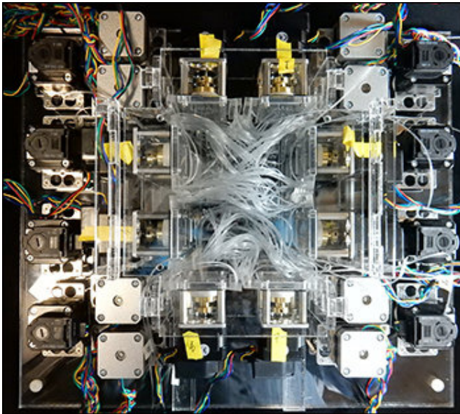
VIIBRE's first 96-Channel MicroFormulator as it is being prepared for shipment to AstraZeneca in January 2016. Credit: Vanderbilt University
