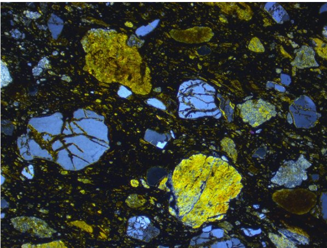
Thin section view of meteoritic ejecta deposit site 1. Note fractured quartz and pervasive fabric. Field of view 4 mm XPolars. Credit: Simon Drake
