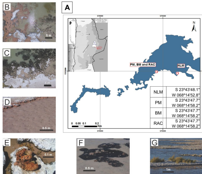
Site location and images showing systems studied. (A) Aerial view of Laguna La Brava indicating the sampling sites. (B) Aerial view of NLM (scale bar 5m). (C) Aerial view of microbialite site. (D) Detail of B, showing NLM (scale bar 0.5m). (E) Top view showing detail of pink mat (PM; scale bar 0.1m). (F) View of black mat (BM, scale bar 0.5m). (G) View from the side of Distichlis spicata (Gramineae), with underground rhizome-associated concretions not visible, scale bar 1m). Credit: Farias et al (2017)
