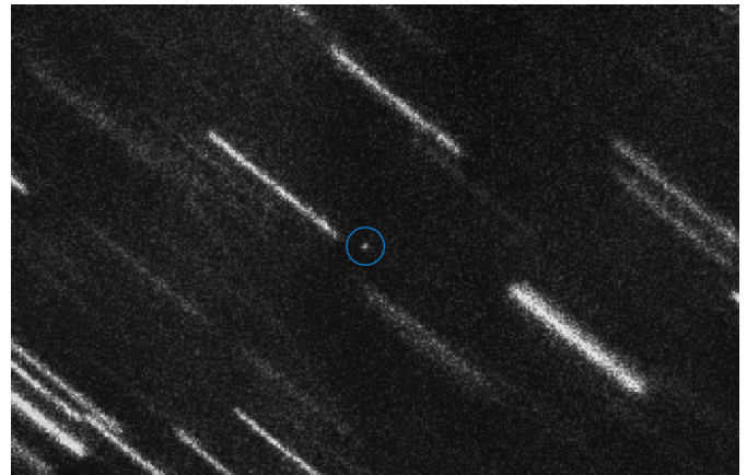
Asteroid 2012 TC4 glides across a field of background stars in this animation taken on Oct. 11, 2017, by the 3.3-foot (1.0-meter) Kiso Schmidt telescope in Nagano, Japan. Credit: Kiso Observatory, University of Tokyo
