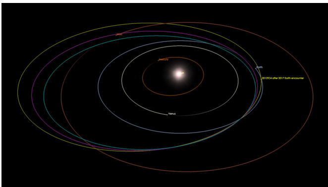
2012 TC4's heliocentric orbit has changed due to the 2012 and 2017 close encounters with Earth. The cyan
