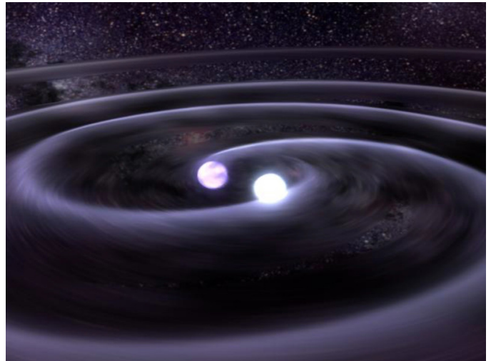
Artist's conception of a binary white dwarf system. Credit: Tod Strohmayer (GSFC), CXC, NASA, Illustration: Dana Berry (CXC)
