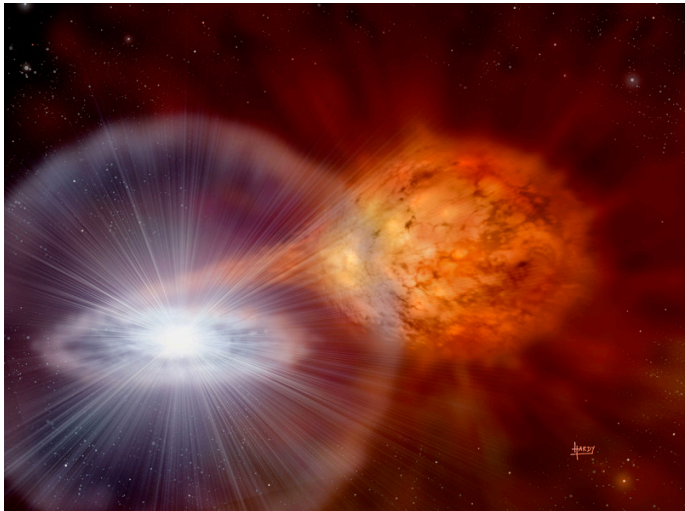
Artist's conception of a white dwarf slowly accreting matter from a companion star. Credit: David A. Hardy & PPARC
