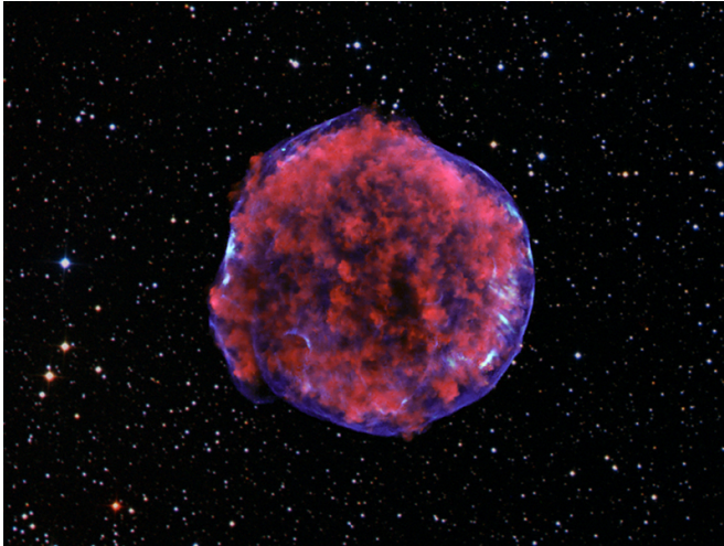
The remnant of Tycho's supernova as seen in X-rays, showing the expanding shock wave. Credit: X-ray: NASA/CXC/Rutgers/K.Eriksen et al.; Optical: DSS
