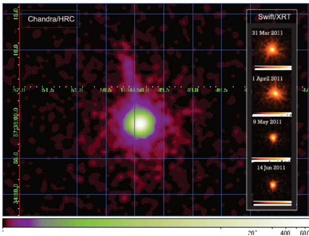
The Chandra/HRC (0.3-10 keV) image of the Swift J1644+57 field of a view (FOV) was observed on 2011 April 4 (MJD=55655) with the 15 ks exposure. Evolution of the Swift/XRT (0.3 - 10 keV) image is plotted in the incorporated vertical panels which clearly demonstrate the outburst decay phase of Swift J1644+57. Credit: Elena Seyfina
