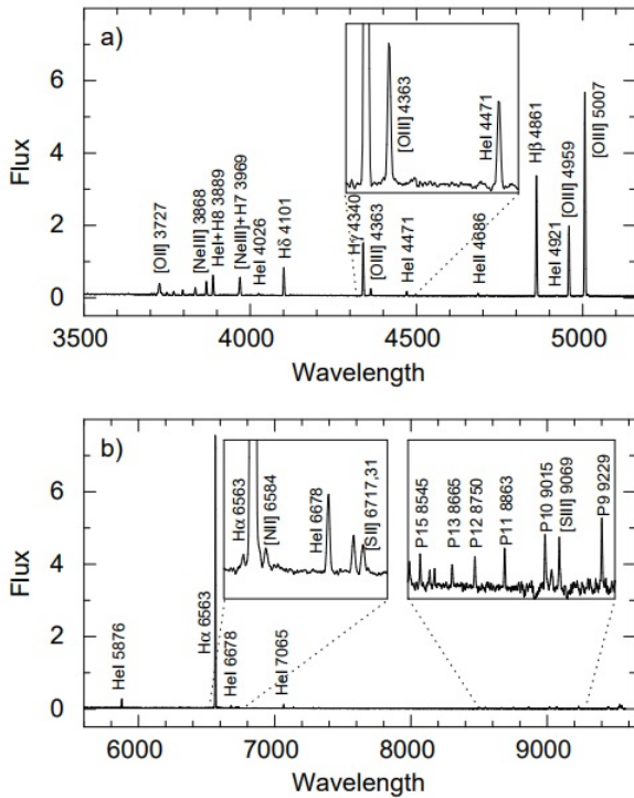
The rest-frame LBT spectrum of J0811+4730 uncorrected for extinction. Credit: Izotov et al., 2017.
