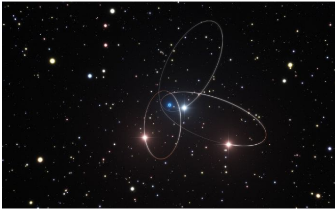
Artist's impression of the orbits of three of the stars very close to the supermassive black hole at the center of the Milky Way. Credit: ESO/M. Parsa/L. Calçada
