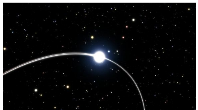
Artist's impression of part of S2's orbit around the supermassive black hole at the center of the Milky Way. Credit: ESO/M. Parsa/L. Calçada
