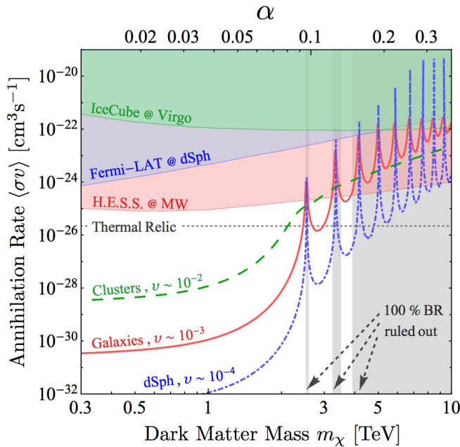
The annihilation rates have a signature non-monotonic velocity dependence over and above the resonances, e.g., for DM mass larger than 4 TeV the galactic annihilation rate (solid line) exceeds that in clusters (dashed line) and dwarf galaxies (dot-dashed line). Credit: Anirban Das, Basudeb Dasgupta
