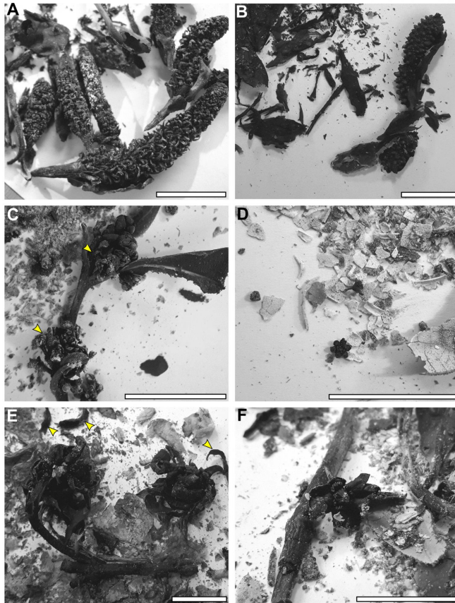
Figure 1 from Hudspith and Belcher: Grayscale photographs of post-burn residues containing char and ash from flowers and associated vegetative material. A: Spikes of Anemopsis californica . B: Spadix of Spathiphyllum wallisii flowers. C: Laurus nobilis flowers clustering in leaf axils (see arrows). D: Differential charcoal production of small isolated charred Cinnamomum camphora flowers compared to ashed leaves, tested under the same conditions. E: Intact charred Schisandraceae: Calycanthus occidentalis flowers; even detached tepals remain as char post-burn (see arrows). F: Intact charred Schisandraceae: Illicium cf. henryi flower. Scale bar in all images is 20 mm. Credit: Geology , Victoria A. Hudspith and Claire M. Belcher
