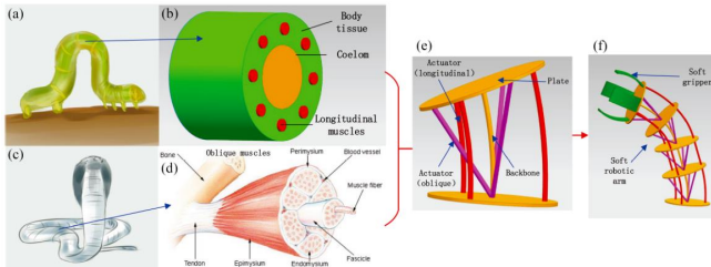
The hybrid structure of the space soft robot for OOS. Credit: ©Science China Press
