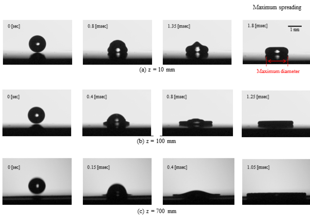
Time progresses from the left image to the right image, where the far-right column of images represents drops exhibiting maximum spreading. (a) release height of the droplet z=10 mm, (b) z=100 mm, (c) z=700 mm. Credit: Assistant Professor Yukihiro Yonemoto
