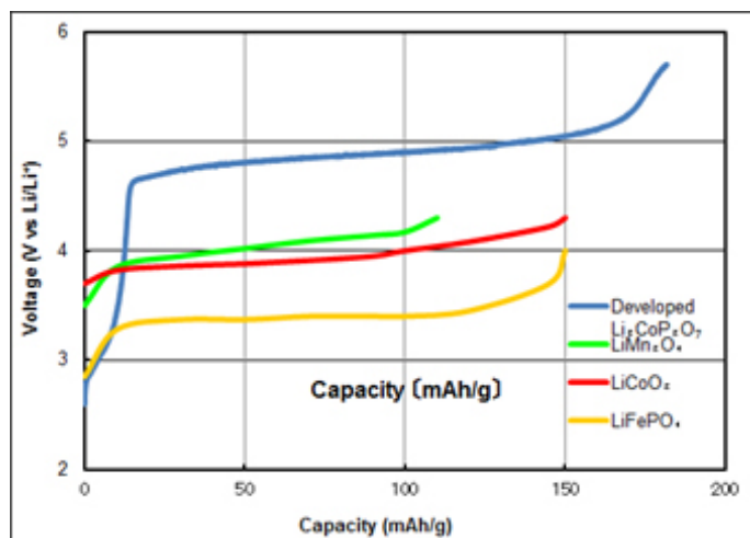
Fig. 2. Comparison of the energy densities of the new cathode material versus conventional cathode materials. Credit: Fujitsu
