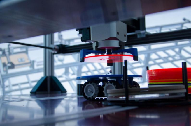
Smart Factory 4.0: processed blanks are lifted onto an automated guided vehicle (AGV). Credit: Fraunhofer IPK
