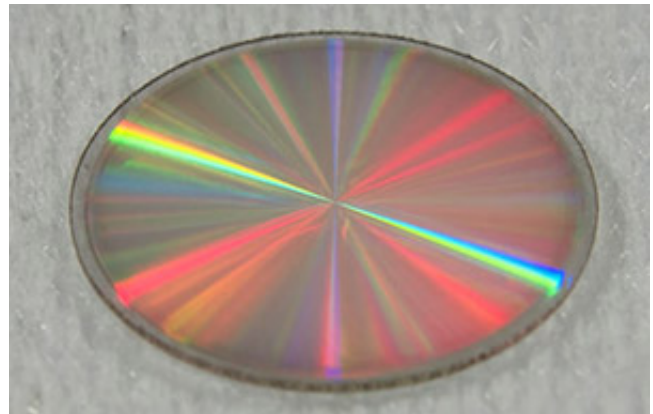
Photograph of a one centimetre large diamond coronagraph. Credit: Uppsala University
