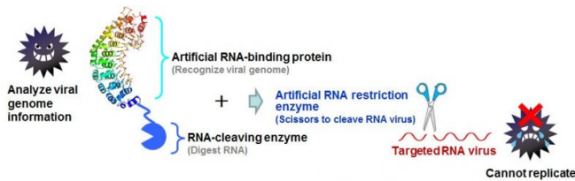
Figure. Analyse virus gene information and create an artificial RNA restriction enzyme. Viruses cannot replicate as their gene information is cleaved (which means virus cannot cause diseases). This technique can be applied to all kinds of RNA viruses both for animals and plants. Credit: Okayama University
