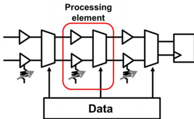
Figure1: Time Domain Neural Network
