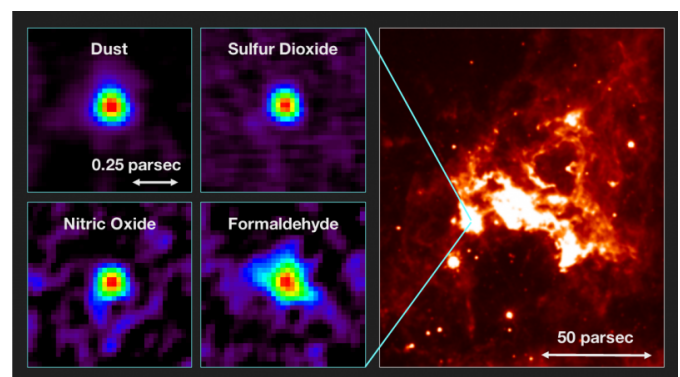
Left: Distributions of molecular line emission from a hot molecular core in the Large Magellanic Cloud observed with ALMA. Emissions from dust, sulfur dioxide (SO 2 ), nitric oxide (NO), and formaldehyde (H 2 CO) are shown as examples. Right: An infrared image of the surrounding star-forming region (based on the 8 micron data provided by the NASA/Spitzer Space Telescope). Credit: T. Shimonishi/Tohoku University, ALMA (ESO/NAOJ/NRAO)
