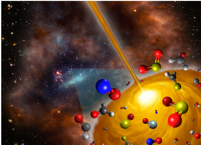
Artist's concept image of the hot molecular core discovered in the Large Magellanic Cloud. Credit: FRIS/Tohoku University. The figure is a derivative work of the following sources (ESO/M. Kornmesser; NASA, ESA, and S. Beckwith (STScI) and the HUDF Team; NASA/ESA and the Hubble Heritage Team (AURA/STScI)/HEI
