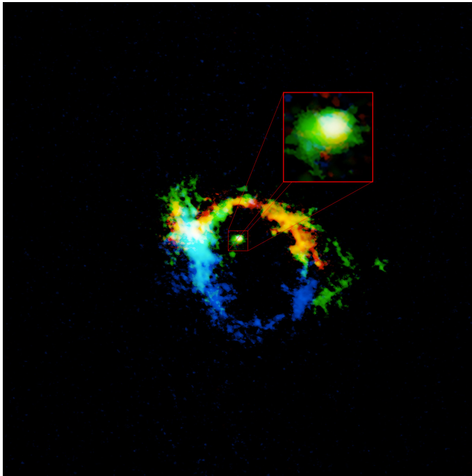
ALMA image of the central region of galaxy NGC 1068. The torus of material harboring the supermassive black hole is highlighted in the pullout box. This region, which is approximately 40 light-years across, is the result of material flung out of the black hole's accretion disk. The colors in this image represent the motion of the gas: blue is material moving toward us, red moving away. The areas in green are low velocity and consistent with rotation around a black hole. The white in the central region means the gas is moving both toward and away at very high speed, the conditions illustrated in the artist impression. The outer ring area is unrelated to the black hole and is more tied to the structure of the central 1,000 light-years of the host galaxy. Credit: Gallimore et al.; ALMA (ESO/NAOJ/NRAO); B. Saxton (NRAO/AUI/NSF)
