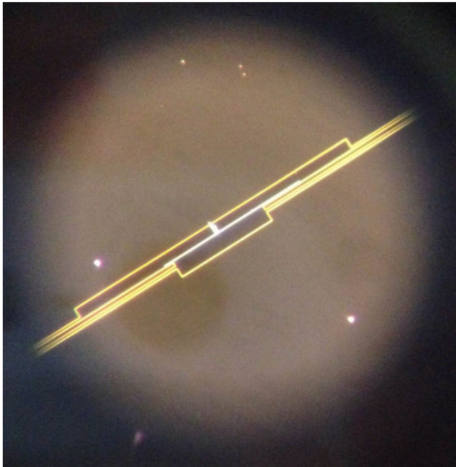
The tuneable microwave single-photon source. Credit: National Physical Laboratory
