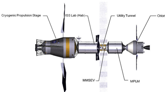
Concept for the design of the ISS-Derived Deep Space Habitat. Credit: NASA
