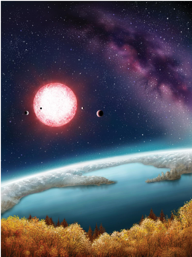
Kepler-186f, seen here in an artist's rendering and discovered in 2014 by a team of astronomers including SF State's Stephen Kane, is one of more than 200 "exoplanets" that researchers say lie within the "habitable zone" of their stars and could potentially have life. Credit: Danielle Futselaar
