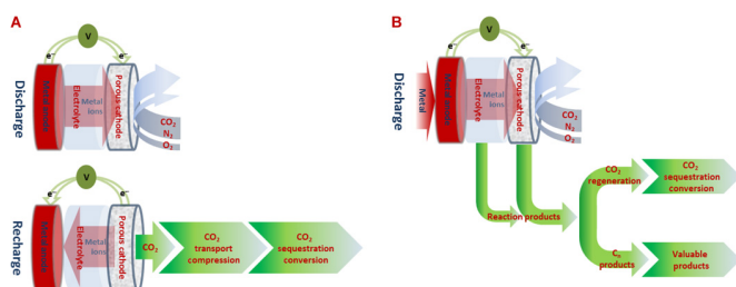
Architectures of metal/CO 2 electrochemical cells as capture systems. Credit: Science Advances 20 Jul 2016: Vol. 2, no. 7, e1600968. DOI: 10.1126/sciadv.1600968
