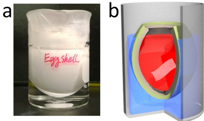
(a) Photo of the experimental setup using an eggshell as a reactor. (b) Illustration of the reactor system. Credit: Meng et al. ©2016 American Chemical Society
