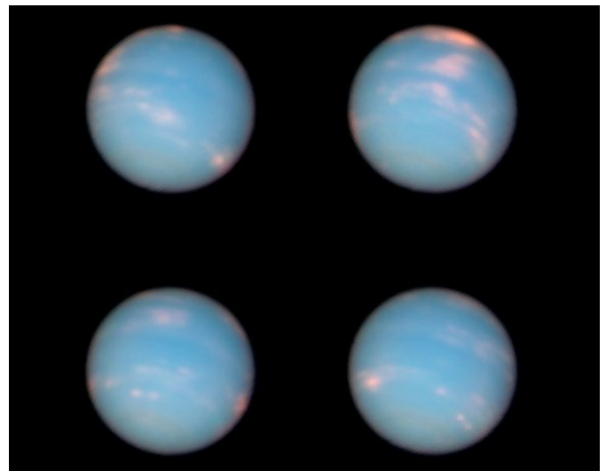
Four images of Neptune taken a few hours apart by the Hubble Space Telescope on June 25-26, 2011. Credit: NASA, ESA and the Hubble Heritage Team (STScI/AURA)
