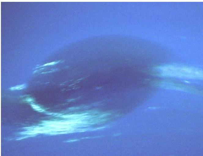
Neptune Great Dark Spot in high resolution. Credit: NASA/JPL
