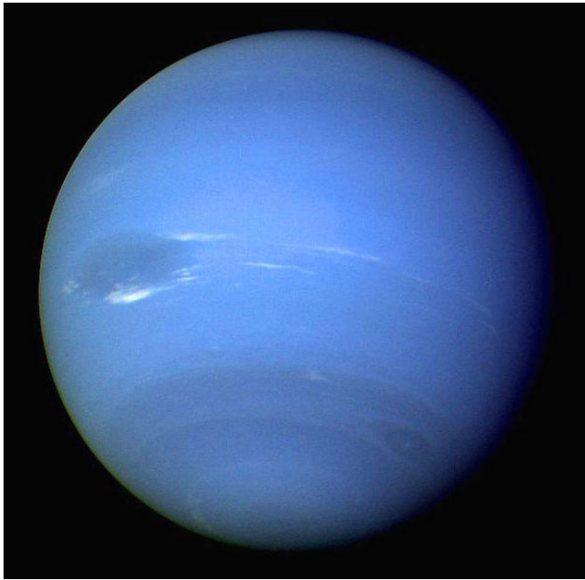
Neptune photographed by Voyager 2. Credit: NASA/JPL
