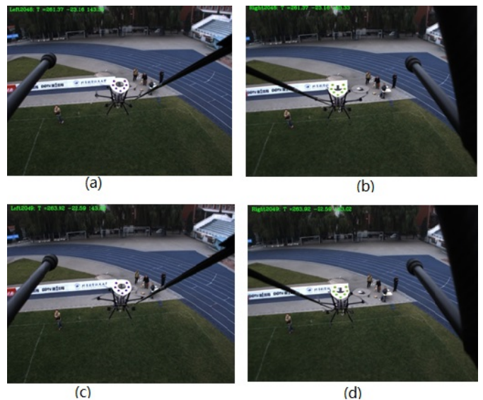
The left frames captured on-board and the reprojection result on the corresponding right frame. (a) and (c) the feature extraction results on images captured with left camera; (b) and (d) relative projection result on images captured with right camera. Credit: ©Science China Press
