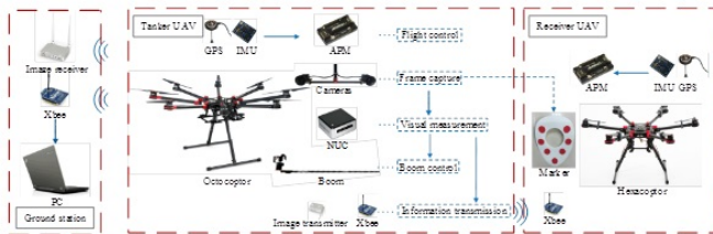
Architecture of binocular vision-based UAVs autonomous aerial refueling platform. Credit: ©Science China Press
