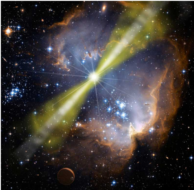
Artist's illustration of a gamma-ray burst. Energy from the explosion is beamed into two narrow, oppositely directed jets. Credit: NASA/Swift/Mary Pat Hrybyk-Keith and John Jones
