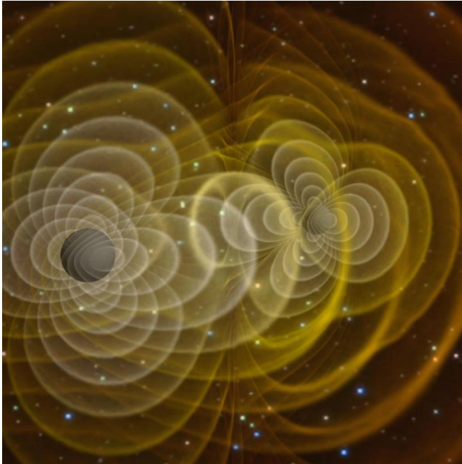
A simulation of two merging black holes, creating gravitational waves. Credit: LIGO.
