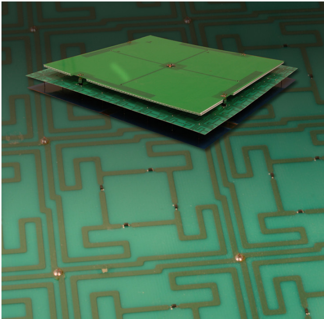
Metamaterial-enabled antenna created by Scarborough and Werner. Credit: Penn State
