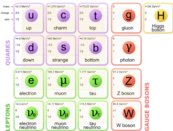
The Standard Model elementary particles. Credit: PBS NOVA/Fermilab/Particle Data Group
