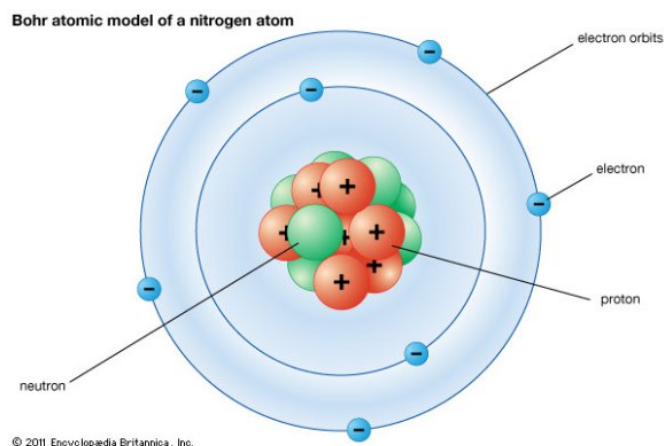
Neils Bohr's model a nitrogen atom. Credit:
