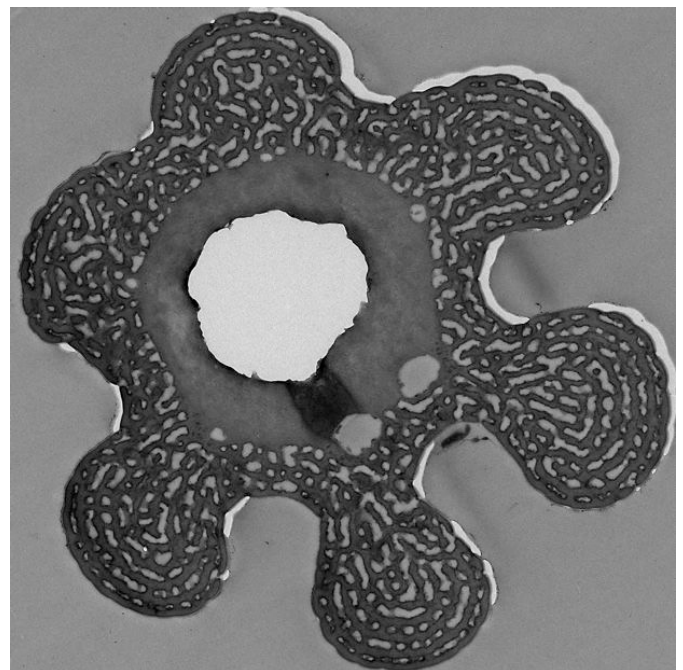
A microscopic image of a multilayer nanostructure inside a tarantula's hair that is responsible for its vibrant blue color. Credit: Scripps Institution of Oceanography, UC San Diego
