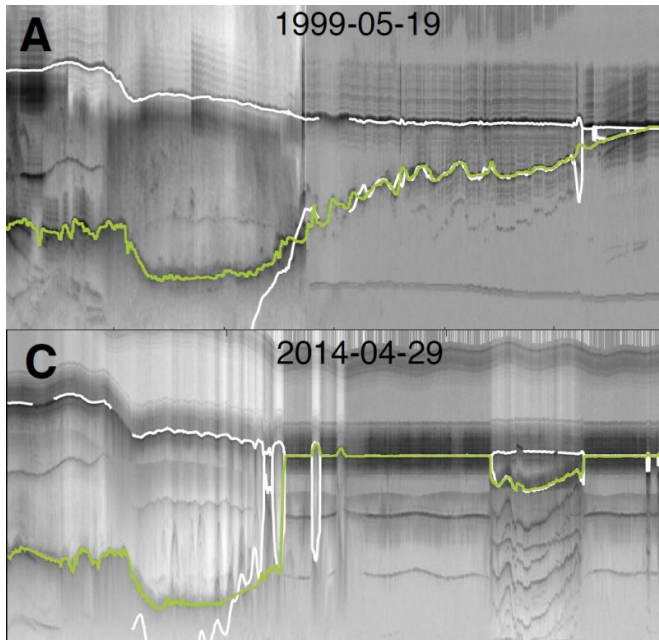
Radar depth-sounder data from before and after the breakup of the Zachariæ Isstrøm ice shelf. The green line reveals the ice bottom, and loss of ice between 1999-2014. The white line represents hydrostatic equilibrium estimates of the ice bottom. Credit: University of Kansas
