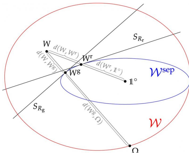
This figure illustrates the test for causal nonseparability, which can determine whether any quantum processes is causally nonseparable. Credit: Araújo, et al.
