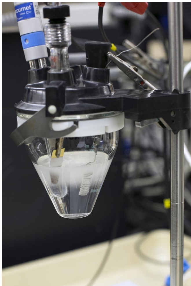
A working cell from Switzer's research, with gas evolution. Credit: Sam O'Keefe, Missouri S&T.
