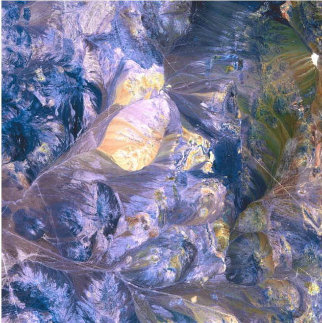
Chile's Atacama Desert captured via the Advanced Spaceborne Thermal Emission and Reflection Radiometer (ASTER) instrument on NASA's Terra satellite on 28 Oct. 2001. Credit: NASA, USGS
