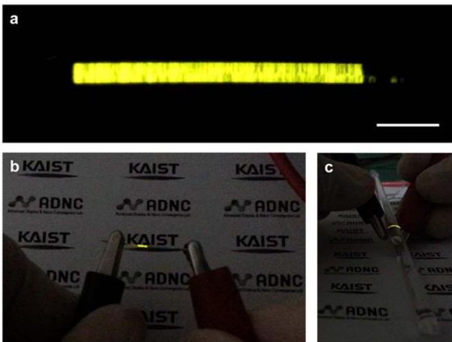
Fiber Based Light Emitting Diodes. Credit: KAIST
