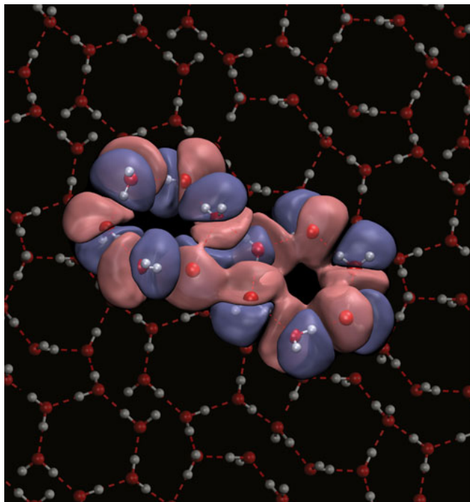
Characteristic hexagonal-ring structure of proton-ordered ice II. Credit: NPL / University of Edinburgh
