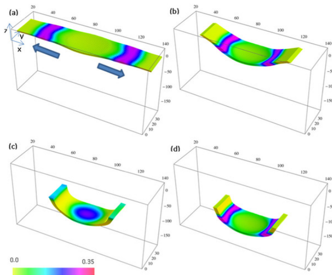
Dynamics of a SP-BZ gel with total concentration of chromophores C_{\text{tsp}}=0.2 . Credit: Scientific Reports , DOI: 10.1038/srep09569
