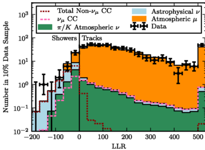
The log-likelihood ratio between shower and track reconstructions for veto-passing events with more than 1500 photoelectrons. Error bars are 68% Feldman-Cousins intervals [51] and show upper limits for bins with no events. The solid-colored distributions are cumulative and result from the best-fit parameters of the distributions shown in Fig. 2. The contribution of muons is determined from a muon control sample. The dotted lines show the total contribution of \nu\mu CC events (pink) and all non- \nu\mu CC events (maroon) from the best-fit distributions of astrophysical and \pi/K neutrinos and are not cumulative with the solid-colored distributions. The last bin contains all overflow events with LLR > 500 . Credit: Phys. Rev. Lett. 114, 171102 – Published 28 April 2015. 10.1103/PhysRevLett.114.171102
