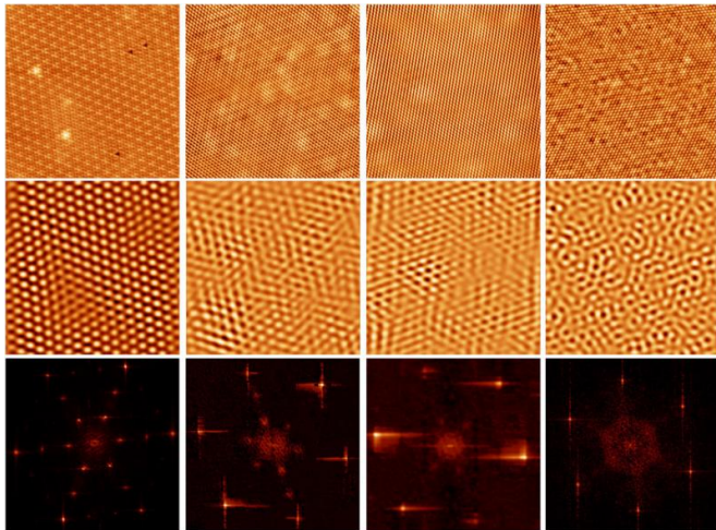
Scanning tunneling microscope images show the configuration of the materials with increased doping (from left to right). Small areas of well-defined charge density wave ordering become visible. Credit: Stephan Rosenkranz
