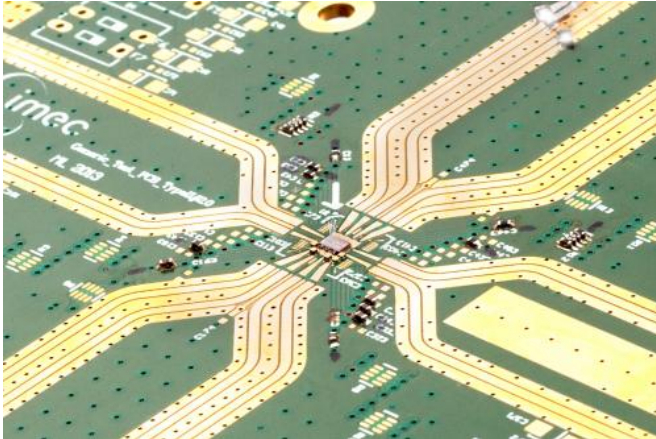
28nm CMOS 79GHz Transceiver Chip for Phase-Modulated Continuous-Wave Radar.
