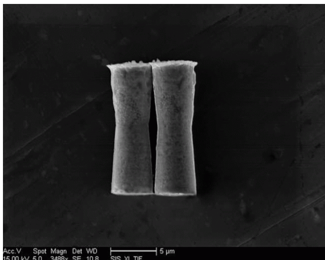
Scanning electron microscopy image of the micromotors. Credit: Jacobs School of Engineering/UC San Diego
