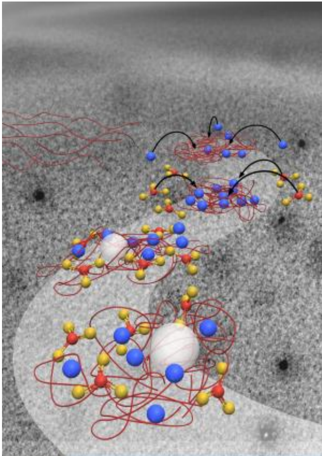
Large charged molecules (red) lure in calcium ions (blue), which position carbonate (yellow and red) and form ACC (white ball). Credit: PNNL
