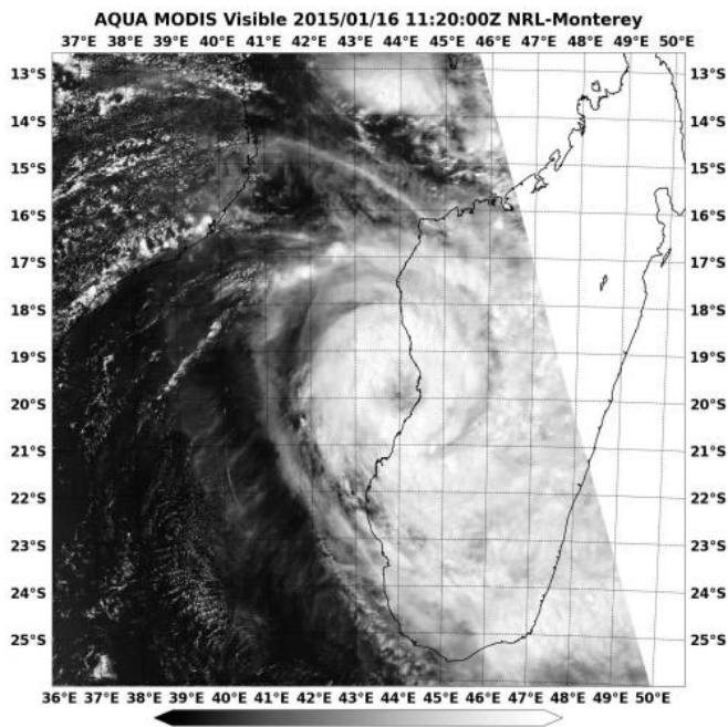
On Jan. 16 at 11:20 UTC NASA's Aqua satellite captured this picture of Tropical Storm Chedza making landfall in southwestern Madagascar. Credit: NASA Goddard MODIS Rapid Response Team
