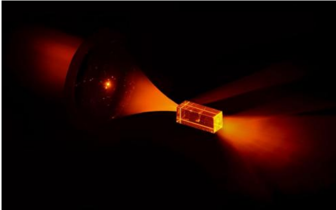
Writing quantum information onto a europium ion embedded in a crystal. Image Solid State Spectroscopy Group, ANU
