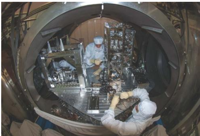
Advanced LIGO will take in huge volumes of data that must be analyzed to determine their meaning. Researchers estimated that ALIGO would generate more than 1 petabyte of data a year, the equivalent of 13.3 years of high-definition video. Credit: MIT/CalTech LIGO
