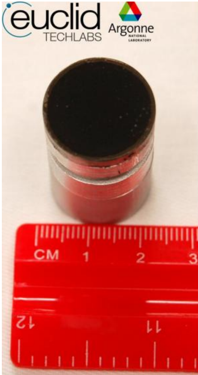
Photograph of a cathode plug for the injector, with an UNCD film deposited on top. Credit: Sergey Baryshev/Euclid TechLabs
