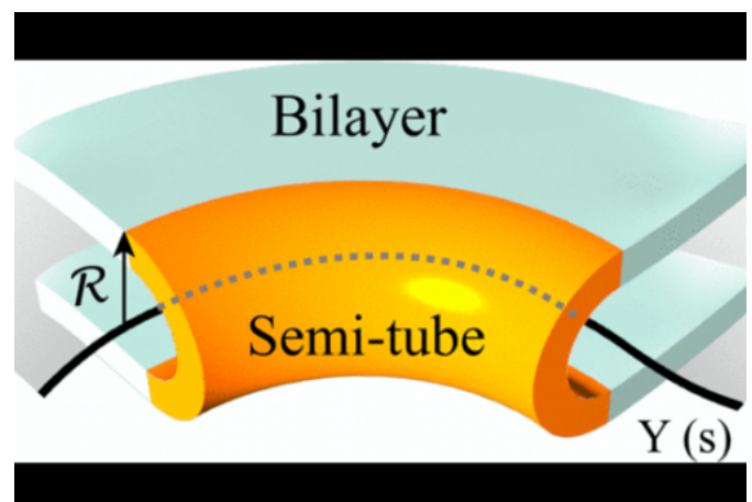
The center of this tube is described by a curve that forms the boundary of a mathematical surface (gray) describing the sheet. Credit: Courtesy PRL
