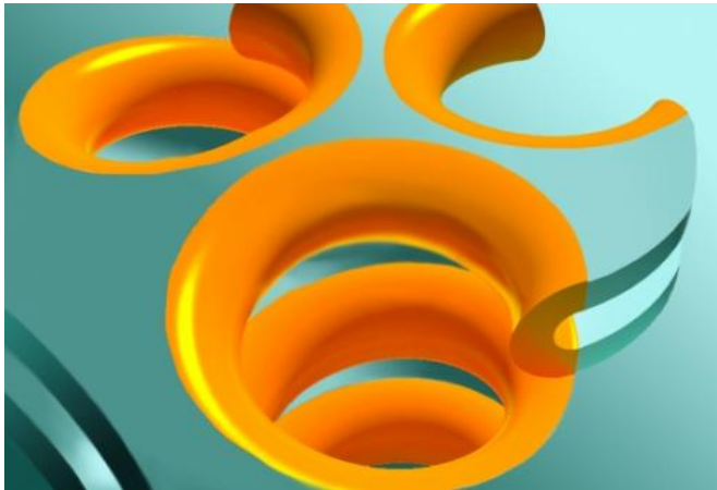
Artist's rendering of Terasaki spiral ramps, helices that connect stacks of evenly spaced sheets in the rough endoplasmic reticulum. Credit: Jemal Guven
