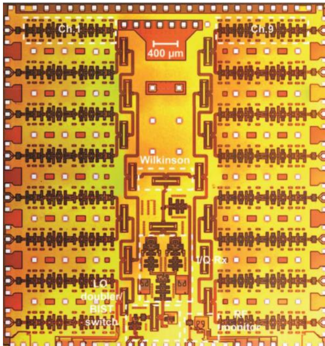
Micrograph of 16-element receiver chip (5.5 5.8 mm 2 ) from "A 77-81 GHz 16-Element Phased-Array Receiver with +/-50° Beam Scanning for Advanced Automotive Radars".
